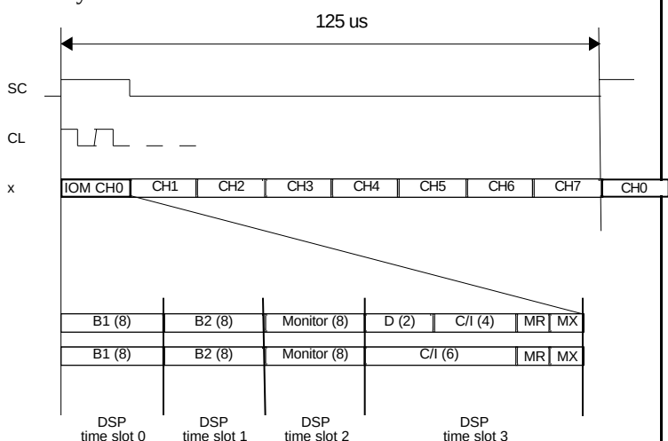
Figure 4-1 IOM-2 Line-Card Mode Interfacing DCL=4.096MHz
